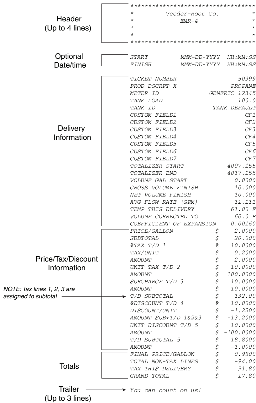
Figure 18. Delivery Ticket Format
