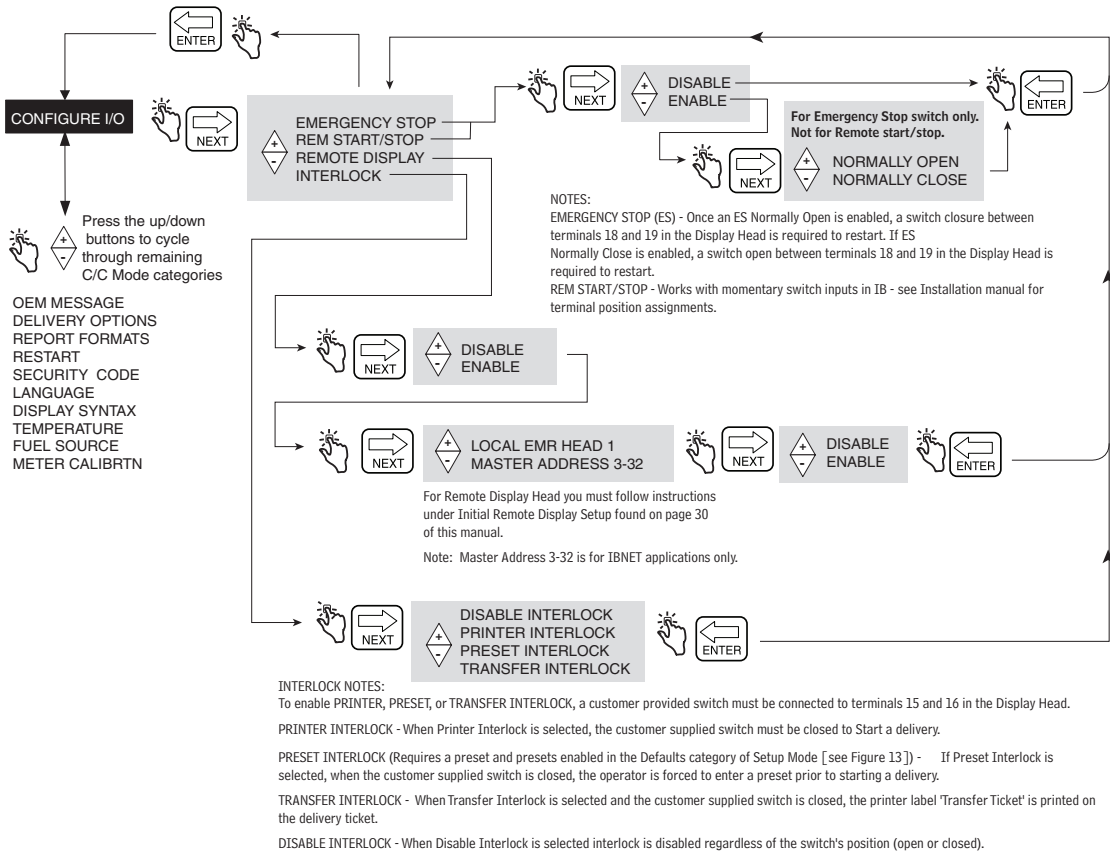
Figure 45. Configure I/O Setup
