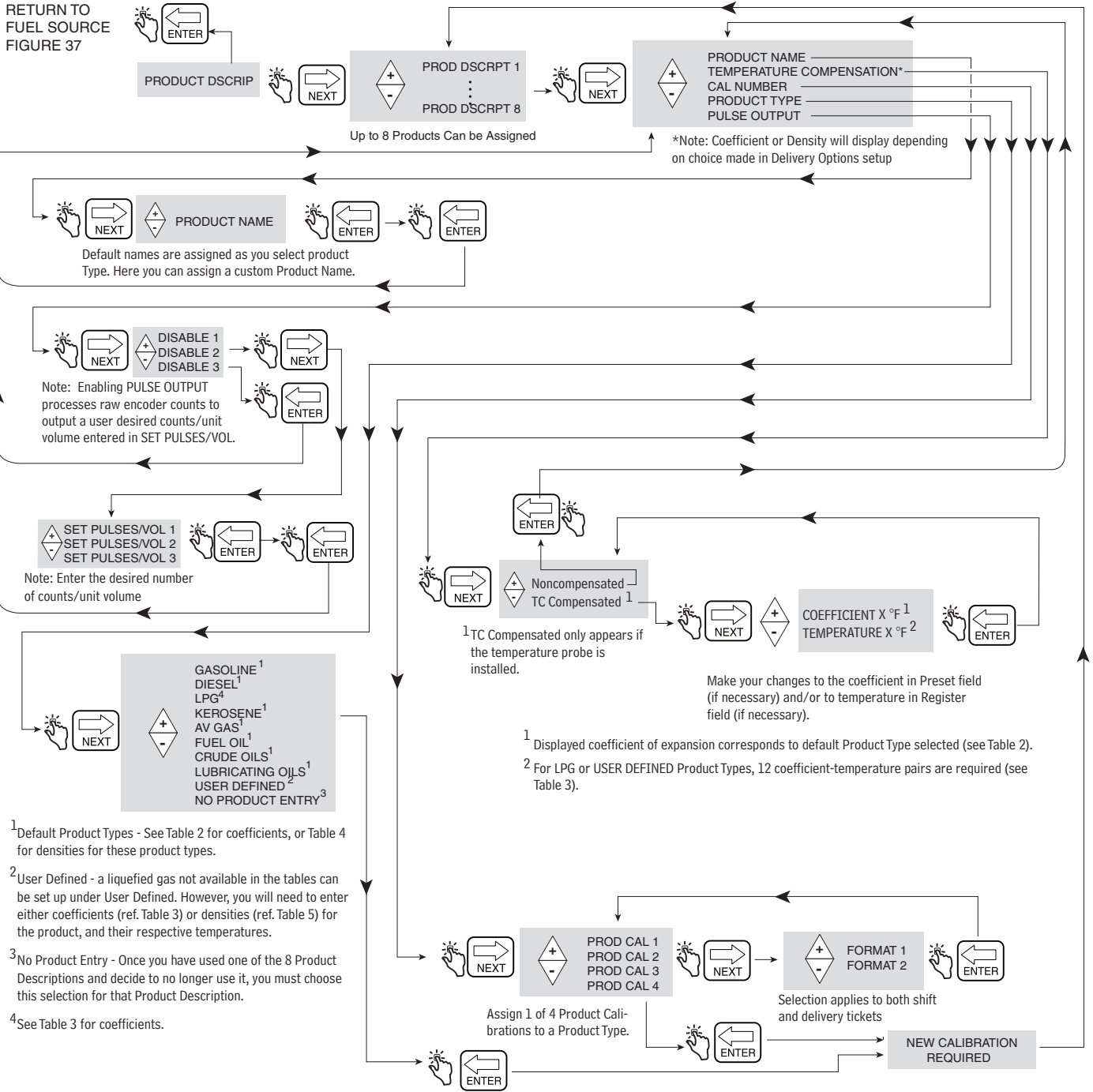
Figure 40. Product Description Setup
